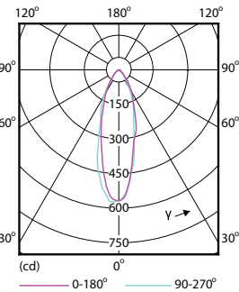
Light Distribution Diagram - Corepro LEDspot 3.5-35W GU10 830 36D
