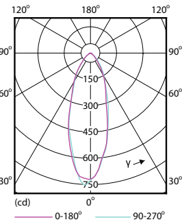
Light Distribution Diagram - Corepro LEDspot 4.6-50W GU10 830 36D
