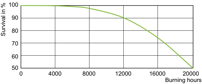
Life Expectancy Diagram - MASTER CityWh CDO-ET Plus 50W/828 E27
