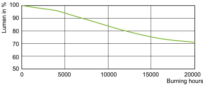
Lumen Maintenance Diagram - MASTER CityWh CDO-ET Plus 50W/828 E27
