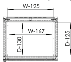
Sectional top view (without bottom plates)
