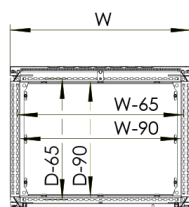
Sectional top view
