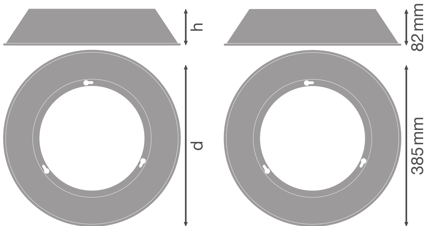
Product line drawing with numbers
