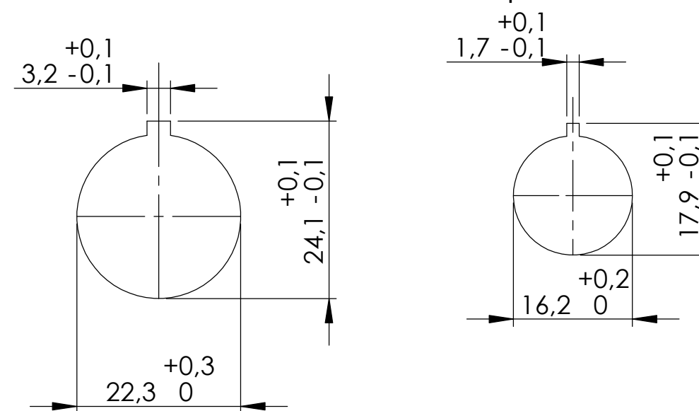
Bohrbild / Hole pattern
