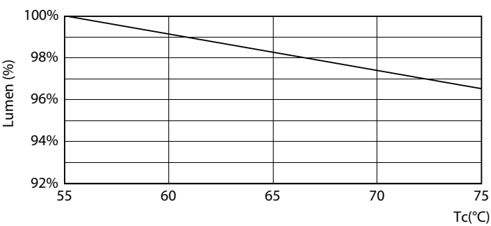
Lumen Maintenance Diagram - MAS LEDtube VLE 600mm HO 8W 865 T8
