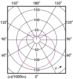
Light Distribution Diagram - CorePro lustre ND 7-60W E14 865 P48 FR
