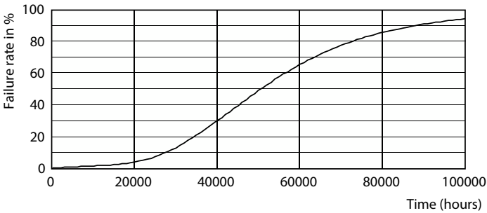
Life Expectancy Diagram - TForce LED SOX 18W B22 840 FR
