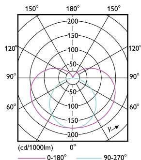
Light Distribution Diagram - TForce LED SOX 18W B22 840 FR
