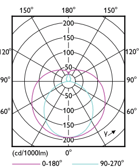
Light Distribution Diagram - MAS LEDtube 1500mm HE 20W 840 T5 EU
