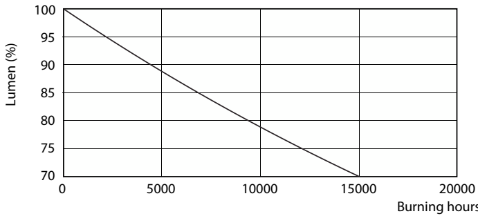
Lumen Maintenance Diagram - CorePro LEDbulb ND 8-60W A60 E27 827 SKT
