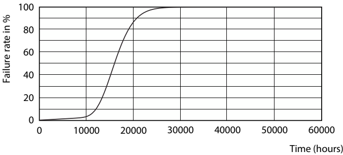
Life Expectancy Diagram - CorePro LEDbulb ND 8-60W A60 E27 827 SKT
