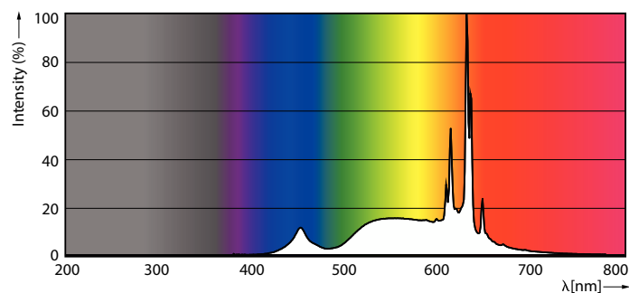
Spectral Power Distribution Colour - MAS VLE LEDLusterDT3.5-40W E27 927P45FRG
