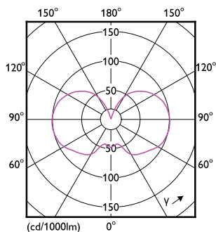
Light Distribution Diagram - MAS VLE LEDLusterDT3.5-40W E27 927P45FRG
