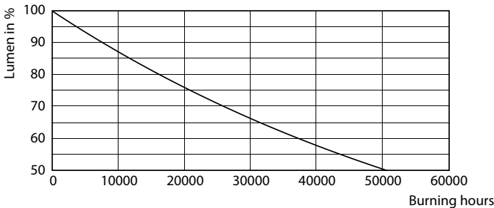
Lumen Maintenance Diagram - MAS VLE LEDLusterDT3.5-40W E27 927P45FRG
