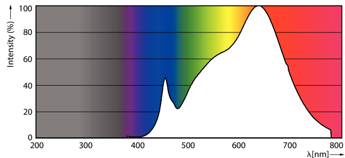
Spectral Power Distribution Colour - MAS LED ExpertColor 6.7-35W MR16 930 10D
