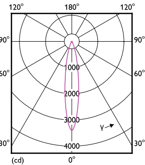
Light Distribution Diagram - MAS LED ExpertColor 7.5-43W MR16 940 24D
