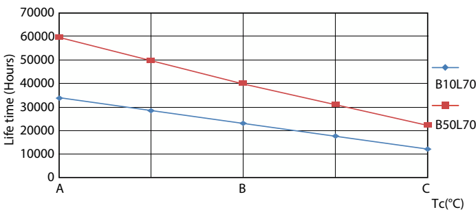
Life Expectancy Diagram - MAS LEDtube VLE 1200mm UO 15.5W 865 T8
