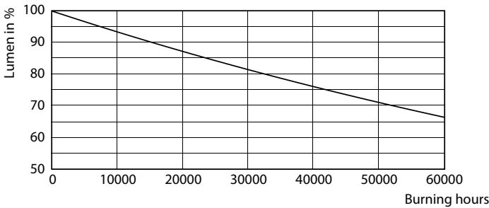
Lumen Maintenance Diagram - TForce LED SOX 28W B22 840 FR
