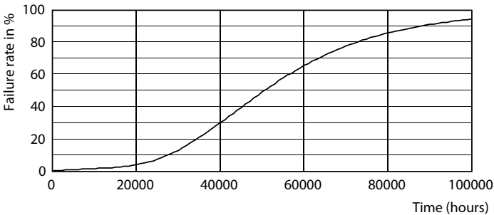
Life Expectancy Diagram - TForce LED SOX 28W B22 840 FR
