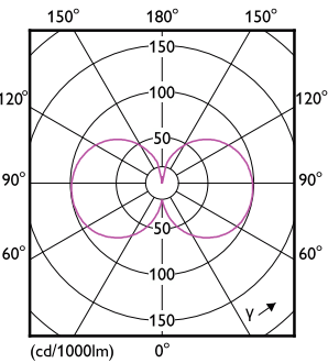
Light Distribution Diagram - CorePro R7S 118mm 7.2-60W 840
