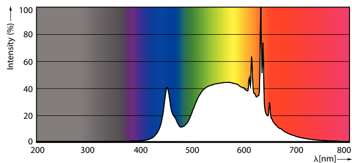
Spectral Power Distribution Colour - MAS LEDBulbND4-60W E27 840 A60 CL G EELA
