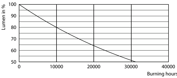
Lumen Maintenance Diagram - MAS VLE LEDBulb D5.9-60W E27 927 A60 FRG
