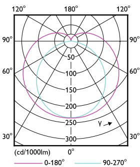
Light Distribution Diagram - MAS LEDtube HF 1500mm HO 20W830 T8
