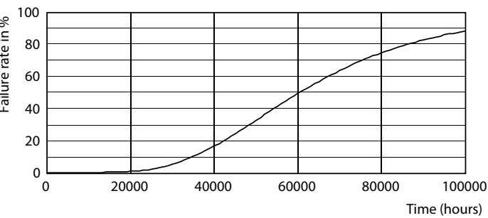
Life Expectancy Diagram - MAS LEDtube HF 1200mm HO 26W 830 T5 OE
