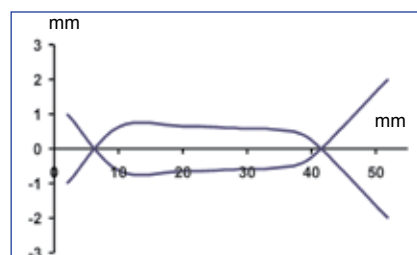
Fixed focus proximity - 50 mm - Detection area
