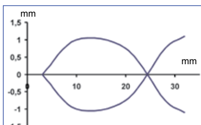
Fixed focus proximity - 30 mm - Detection area
