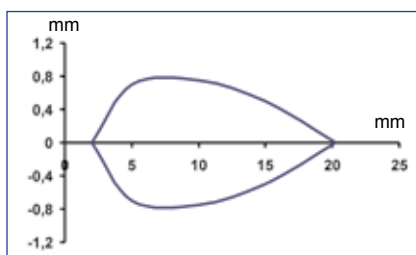
Fixed focus proximity - 20 mm - Detection area
