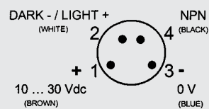
NPN OUTPUT(SR31-0)
