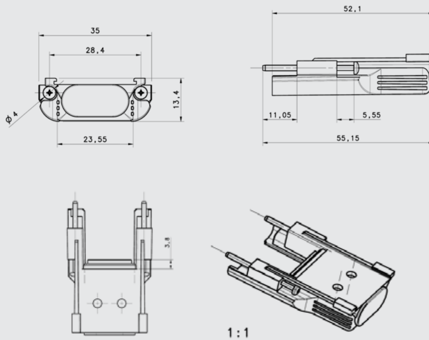
TERMINATOR CAP
