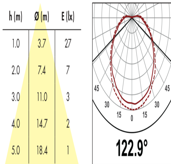
Stralingshoek
