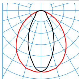
Nextrema G3 TB 80-840 +LV TWP LHT TX150308
