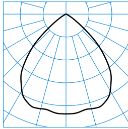
InperiaL G2 C07 BR22 1800-830 01 + RD-PC ■ C0 - C180 TX373307
