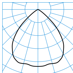
InperlaL G2 C07 BR22 1800-830 01 + RG-PC ■ C0 - C180 TX373306
