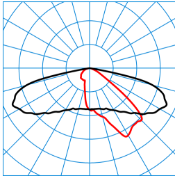
LIQ 50N-AB2L-LRA/2200-722 2G1 ETDD (CLO initial value) TX281093
