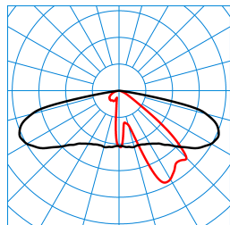
Publisca P2-AB2L-LR/1000-730 2G1S ET (CLO end value) TX301282 DIN 5040: A30 UTE: 1,00 G CEN Flux Code: 34 70 96 100 100
