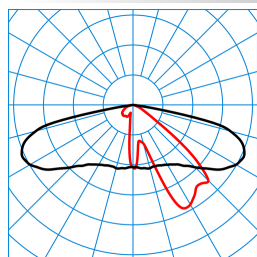
Publisca P2-AB2L-LR/1000-730 2G1S TX047731 DIN 5040: A30 UTE: 1,00 G CEN Flux Code: 34 70 96 100 100
