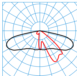
Publisca P2-AB2L-LR/1000-730 2G1S ET (CLO initial value) TX300928 DIN 5040: A30 UTE: 1,00 G CEN Flux Code: 34 70 96 100 100
