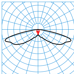
Publisca P1-SB3L/1200-740 2G1S ETDD (CLO initial value) TX300291
