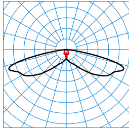
Publisca P1-SB3L/1200-740 2G1S ETDD (CLO end value) TX300968
