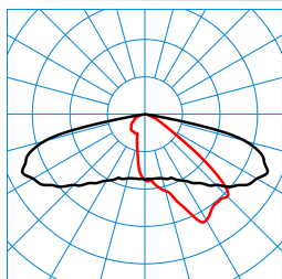
LIQ 50N-AB2L-LRA/2400-727 4G1 ETDD (CLO end value) TX278362
