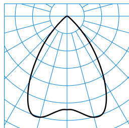
InperiaL G2 C07 BR19 1000-830 03 + RD-PC ■ C0 - C180 TX373457
