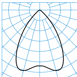
InperlaL G2 C07 BR19 1000-830 03 + RG-PC ■ C0 - C180 TX373455
