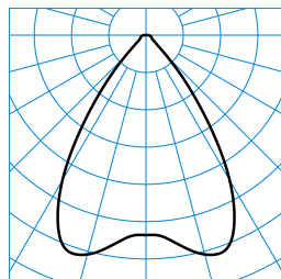
InperiaL G2 C07 BR19 1000-830 03 + ZN-PC ■ C0 - C180 TX373453
