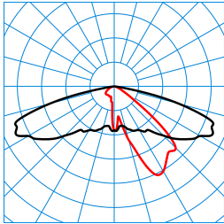
Publisca P1W-AB2L-LR/4600-730 6G1S ET (CLO end value) TX300355 DIN 5040: A30 UTE: 1,00 G CEN Flux Code: 34 72 97 100 100 0 0 0 0
