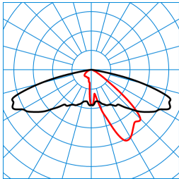
Publisca P1W-AB2L-LR/4600-730 6G1S ET (CLO initial value) TX301629 DIN 5040: A30 UTE: 1,00 G CEN Flux Code: 34 72 97 100 100 0 0 0 0
