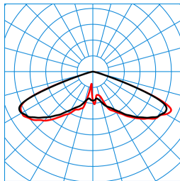
Publisca P1-RB6L-LR/2000-730 3G1S TX047628 ■ C0 - C180 ■ C90 - C270 DIN 5040: A20 UTE: 1,00 J CEN Flux Code: 20 57 98 100 100
