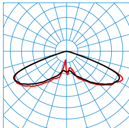
Publisca P1-RB6L-LR/2000-730 3G1S ET (CLO initial value) TX300602 ■ C0 - C180 ■ C90 - C270 DIN 5040: A20 UTE: 1,00 J CEN Flux Code: 20 57 98 100 100
