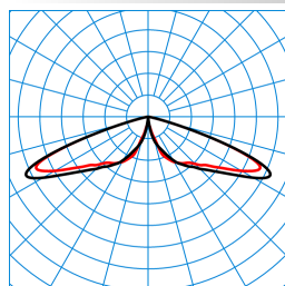
CS 19 100-RB6L/1200-740 2G1S ETDD (CLO end value) TX300055
