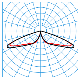
CS 19 100-RB6L/1200-740 2G1S ETDD (CLO initial value) TX300056
