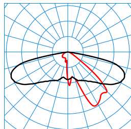
Publisca P2-AB2L-LRA/2200-740 3G1S ET (CLO end value) TX301703 ■ C0 - C180 ■ C90 - C270 DIN 5040: A30 UTE: 1,00 l CEN Flux Code: 34 71 96 100 100
