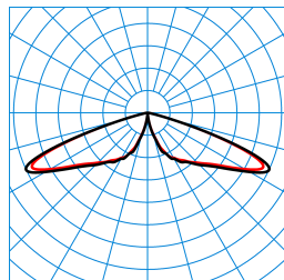
CS 19 100-RB6L/4600-730 4G1S ETDD (CLO initial value) TX300116
