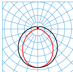
So-TubeAct G3 D/H1 DW 10 ETDD 05 (ACTDISU) TX281409
