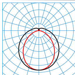
So-TubeAct G3 D/H1 DW 10 ETDD 05 (ACTDICW) TX281414
