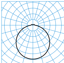
Olisq Act RWD2 DW 40 ETDD8 IP54 + Olisq RWD2 ZDR 1/2 05 (ActDWW) TX428828
