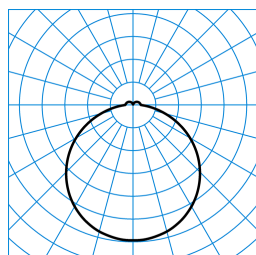
Olisq Act RWD2 DW 40 ETDD8 IP54 + Olisq RWD2 ZDR 1/2 03 (ActDWW) TX427714
