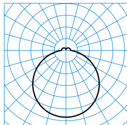
Olisq Act RWD2 DW 40 ETDD8 IP54 (ActDCW) TX376323
