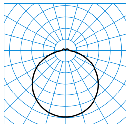
Olisq Act RWD2 DW 40 ETDD8 IP54 + Olisq RWD2 ZDR 1/2 01 (ActDWW) TX426012
