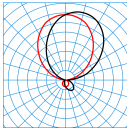
Sanesca W3-S1/R LED5000-830 01 TX371841
