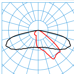
LIQ 50N-AB2L-LRA/5100-722 6G1 ETDD (CLO end value) TX280924
