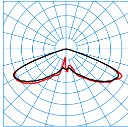
Publisca P2-RB6L-LR/2600-730 3G1S ET (CLO end value) TX301274 DIN 5040: A20 UTE: 1,00 J CEN Flux Code: 20 57 98 100 100
