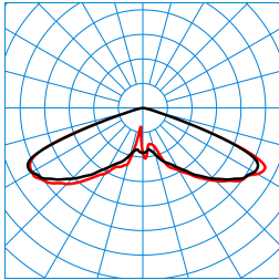
Publisca P2-RB6L-LRA/2400-730 3G1S ET (CLO end value) TX300516 ■ C0 - C180 ■ C90 - C270 DIN 5040: A20 UTE: 1,00 J CEN Flux Code: 20 57 98 100 100
