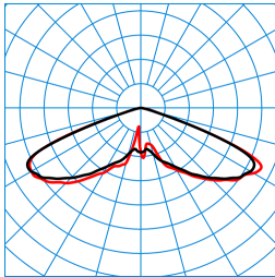
Publisca P2-RB6L-LRA/2400-730 3G1S ET (CLO initial value) TX301569 ■ C0 - C180 ■ C90 - C270 DIN 5040: A20 UTE: 1,00 J CEN Flux Code: 20 57 98 100 100
