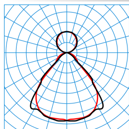
SFlow H2-L MRW LED6400-840 03 TX050993
