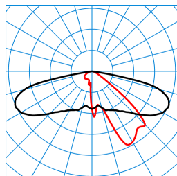
Publisca P1-AB2L-LRA/2600-730 3G1S ET (CLO initial value) TX301860 DIN 5040: A30 UTE: 1,00 l CEN Flux Code: 34 71 96 100 100
