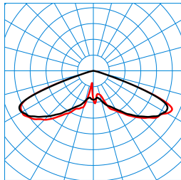
Publisca P2-RB6L-LRA/2600-730 3G1S ET (CLO end value) TX301933 ■ C0 - C180 ■ C90 - C270 DIN 5040: A20 UTE: 1,00 J CEN Flux Code: 20 57 98 100 100
