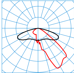
Publisca P1-AB2L/2900-730 4G1S ETDD (CLO end value) TX300792
