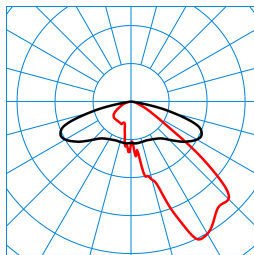
Publisca P2-AB2L-LR/2900-730 4G1S ET (CLO end value) TX300252 DIN 5040: A30 UTE: 1,00 G CEN Flux Code: 35 73 97 100 100 ■ C0 - C180 ■ C90 - C270
