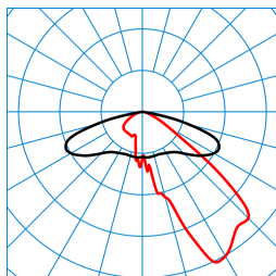
Publisca P2-AB2L-LR/2900-730 4G1S ET (CLO initial value) TX300693 DIN 5040: A30 UTE: 1,00 G CEN Flux Code: 35 73 97 100 100 ■ C0 - C180 ■ C90 - C270
