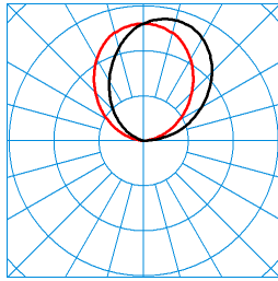
Sanesca W3-S1/R LED5000-830 01 (night light) TX055775
