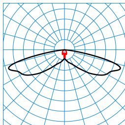
Publisca P1-SB3L/800-740 2G1S ETDD (CLO initial value) TX301032
